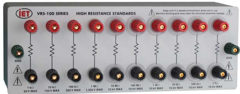
Model VRS-100-10-BP-10kV High Resistance Standards, binding post style, 10 kV option and case ground
